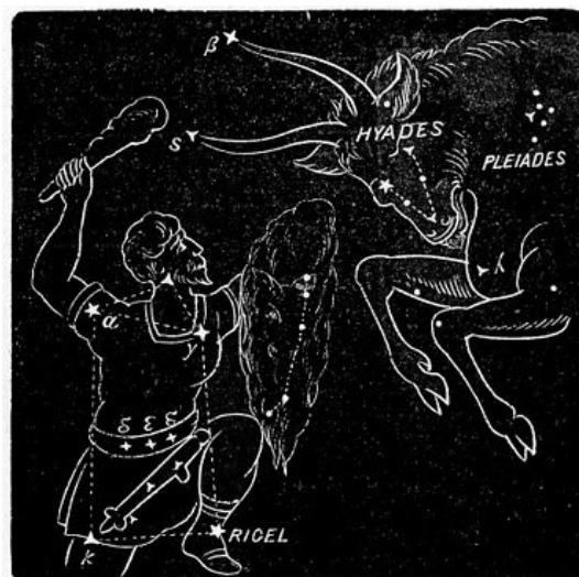
Fig. 26. Orion and Taurus.
